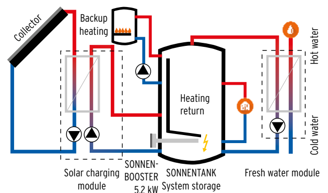
Functional diagram COMFORT Plus HEATING
