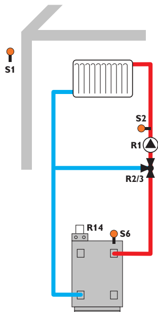
Scheme 2: 1 mixed heating circuit with backup heating (demand)
