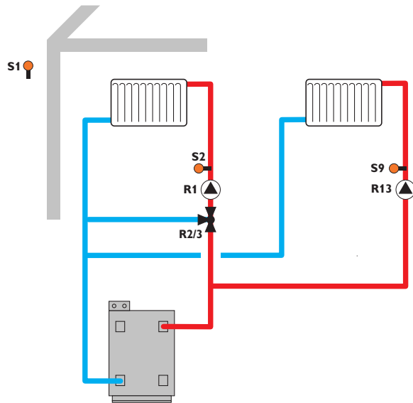
Scheme 6: 1 mixed and 1 unmixed heating circuit
