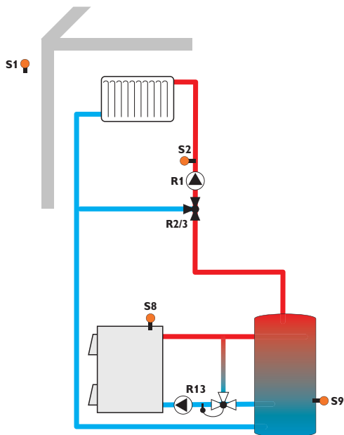
Scheme 8: 1 mixed heating circuit with solid fuel boiler
