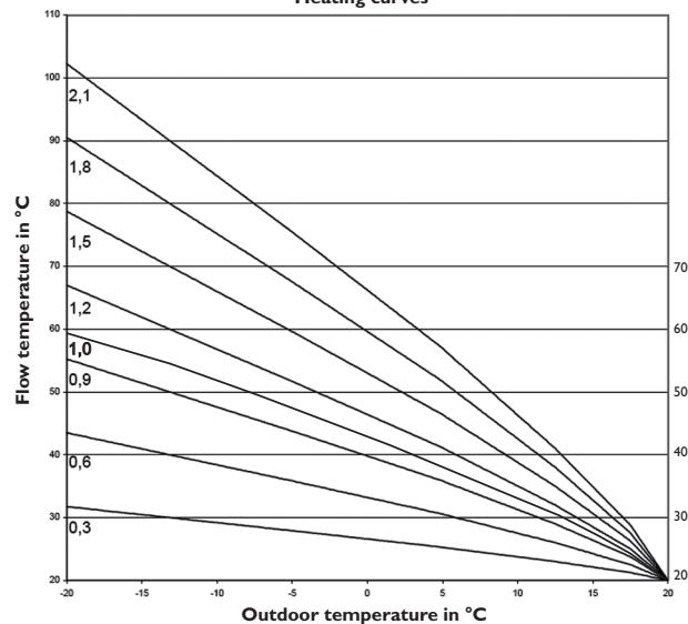
Heating curves
