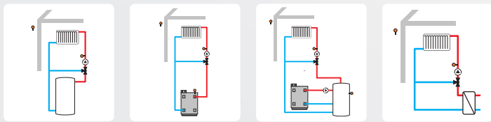
1 mixed heating circuit with external heat source (e.g. district heating) 1 mixed heating circuit with afterheating (demand) 1 mixed heating circuit with afterheating (demand and boiler loading pump) 1 mixed heating circuit with external heat source (e.g. district heating)
