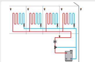
1 mixed heating circuit with 4 zones
