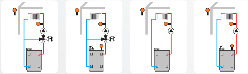
1 mixed heating circuit 1 mixed heating circuit with afterheating (demand) 1 static heating circuit 1 static heating circuit with afterheating (demand)
