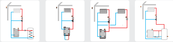
1 mixed heating circuit with DHW heating and afterheating (demand for heating circuit and DHW) 1 mixed heating circuit with DHW heating (e.g. heat pump) 1 mixed and one un-mixed heating circuit with afterheating (demand) 1 mixed heating circuit with solid fuel boiler
