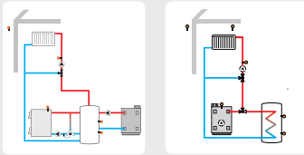
1 mixed heating circuit with solid fuel boiler and afterheating (demand) 1 mixed heating circuit with DHW heating (3-port valve)
