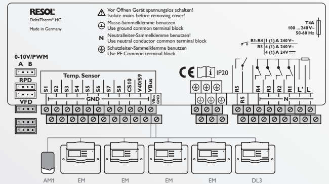
1 mixed heating circuit with external heat source (e.g. district heating) 1 mixed heating circuit with afterheating (demand) 1 mixed heating circuit with afterheating (demand and boiler loading pump) 1 mixed heating circuit with external heat source (e.g. district heating)
